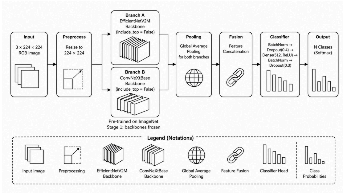
Figure 3.5: ABS Hybrid dual-backbone architecture.
