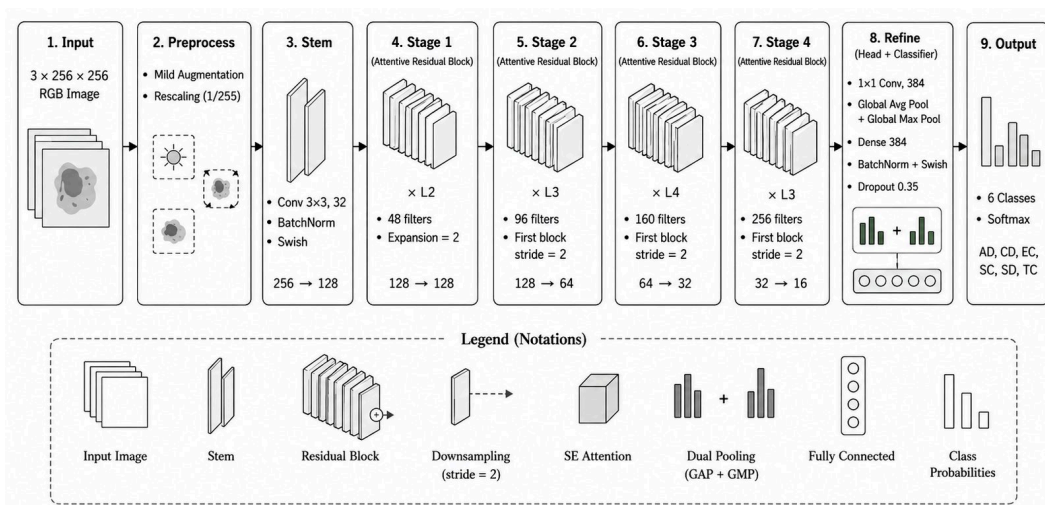
Figure 3.8: TRY NET-8 attentive residual CNN architecture.
