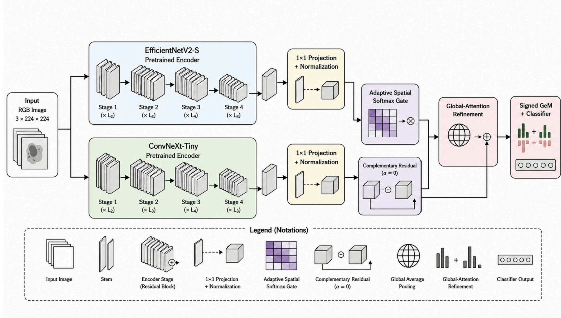
Figure 3.9: UGVNet dual-backbone architecture.
