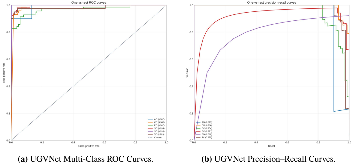
Figure 4.8: Multi-class ROC and Precision-Recall trajectories for the UGVNet architecture.
