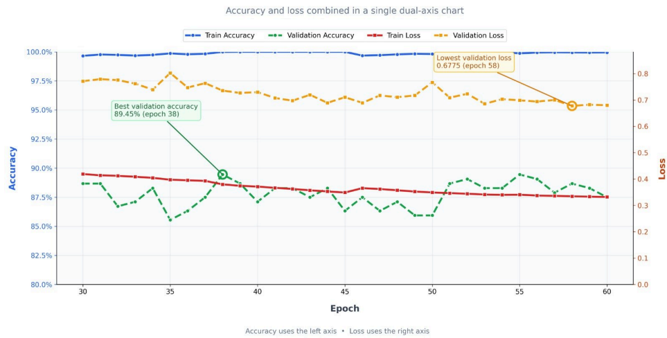
(c) TRY NET-8 training and validation curves.
