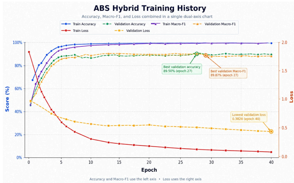
(b) ABS Hybrid training and validation curves
