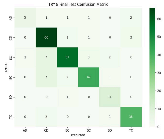
(b) TRY NET-8 test confusion matrix.
