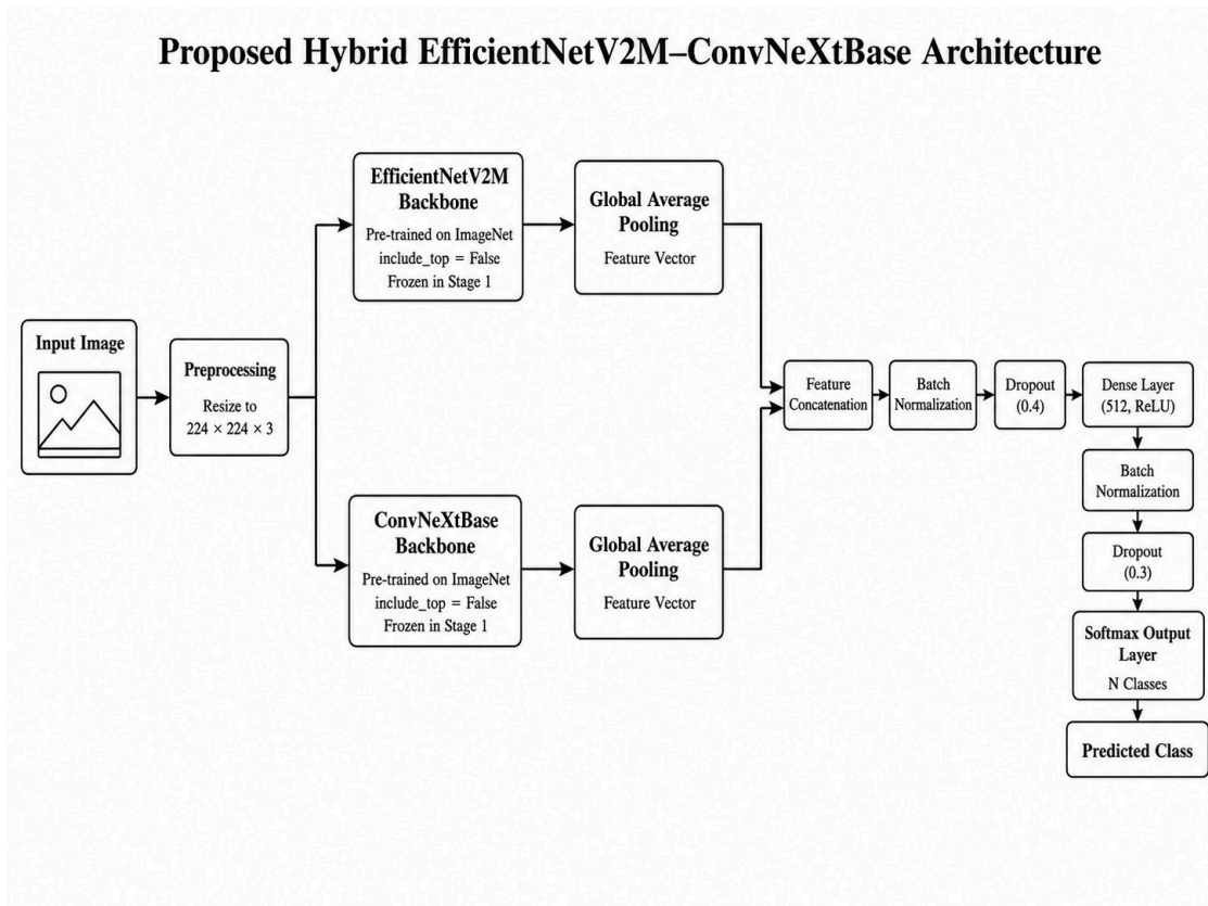
Figure 3.6: ABS Hybrid fusion and classification head.
