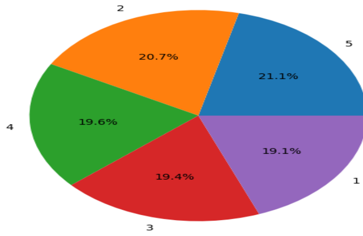
quantity Distribution
