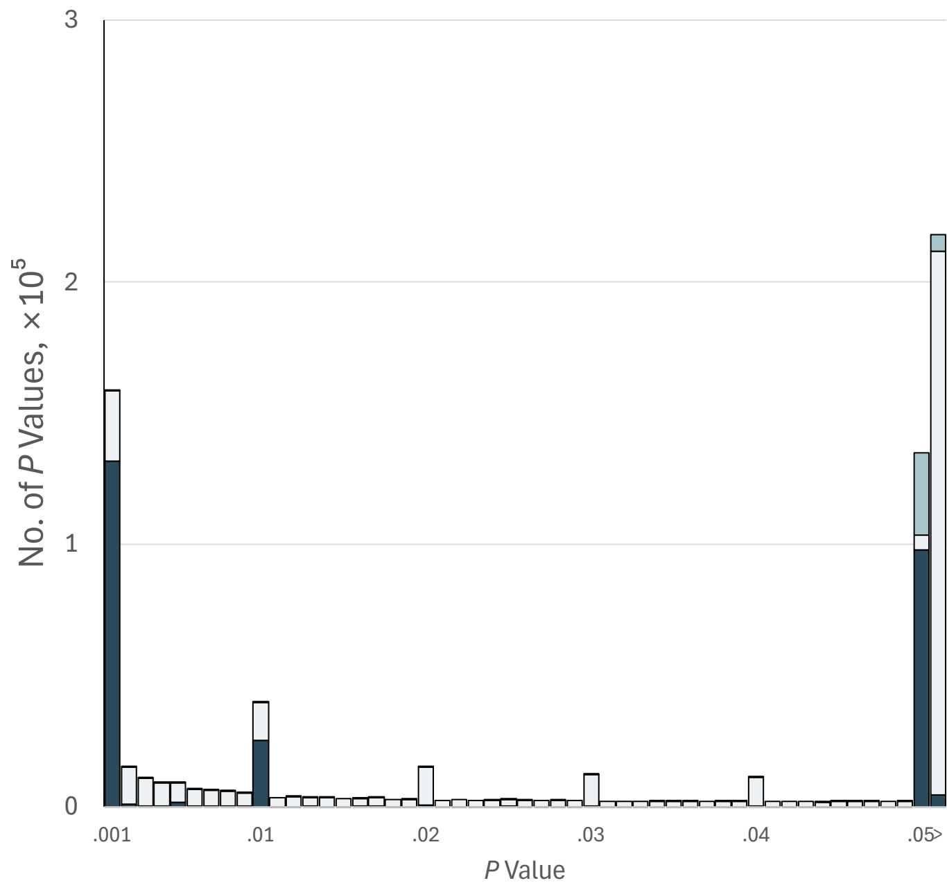
Randomized controlled trial (70 554 articles, 749 824 P values)
