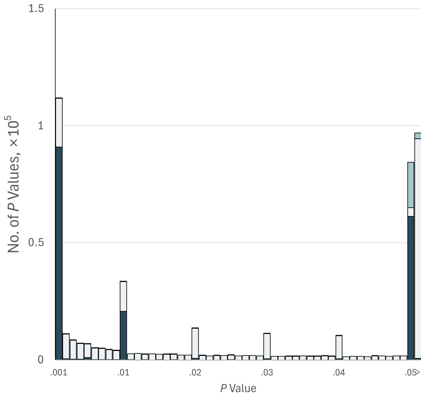
Randomized controlled trial (265 975 articles, 482 045 P values)
