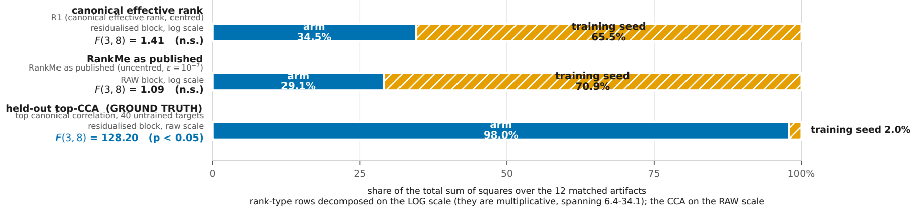
(a) The decomposition: how much of each quantity is the ARM, and how much is the training SEED
