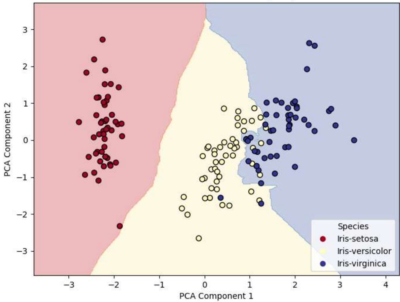
KNN Decision Boundaries (K=5)
