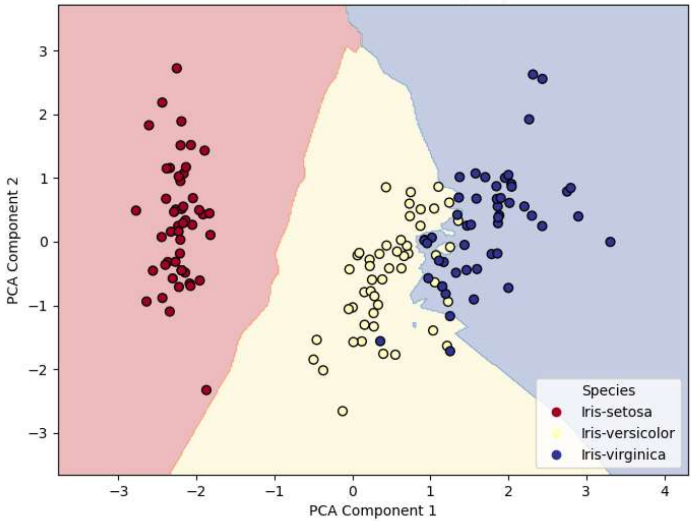
KNN Decision Boundaries (K=3)
