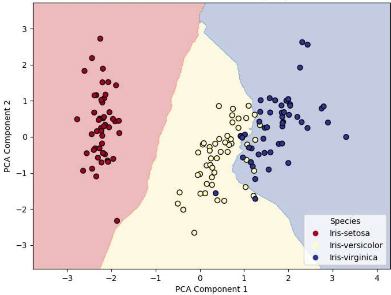
KNN Decision Boundaries (K=7)
