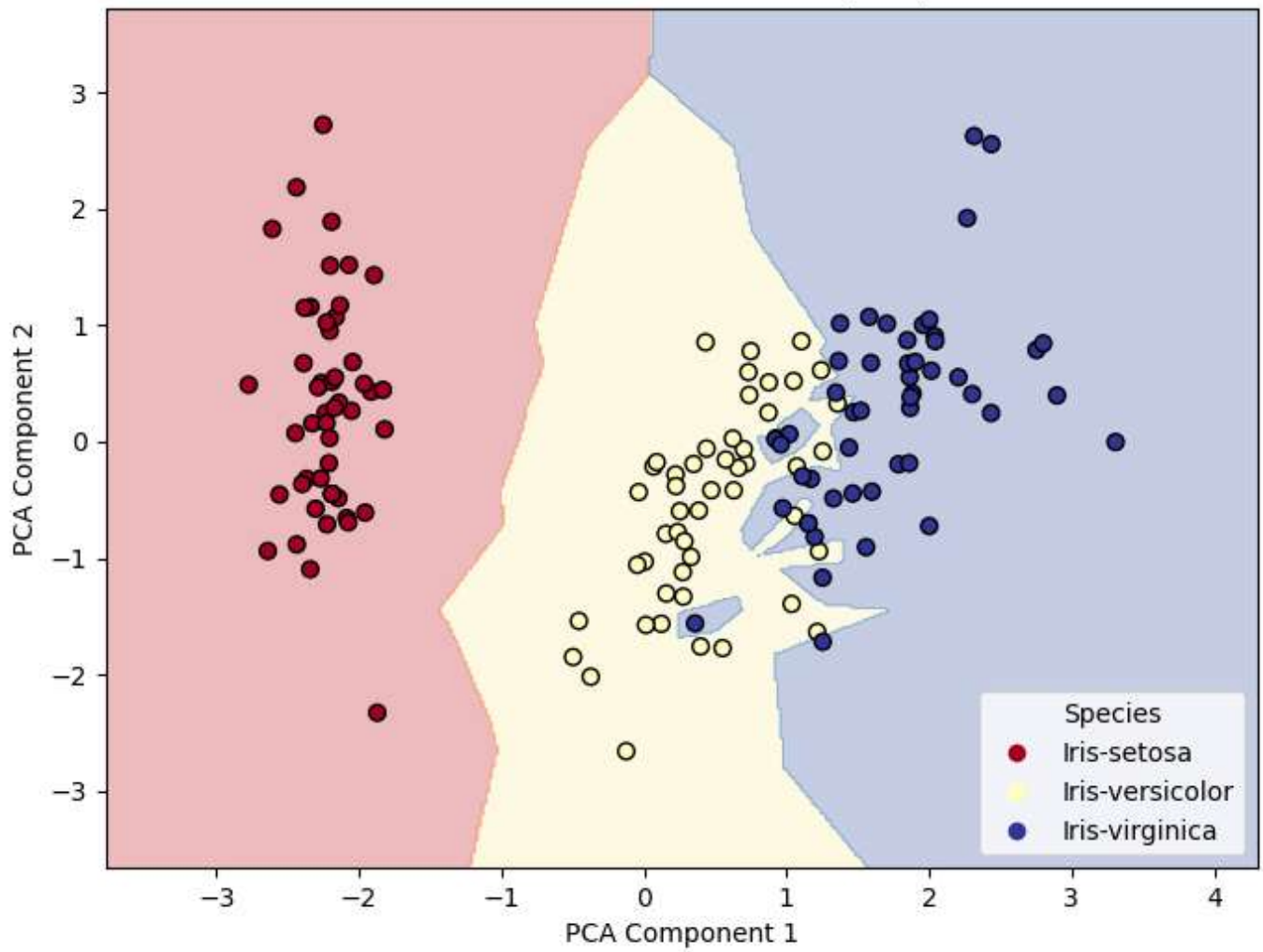
KNN Decision Boundaries (K=1)
