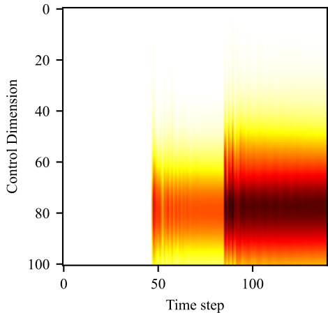
Closed-loop Control Inputs
