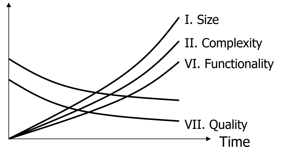
Lehman's Laws of Software Evolution
