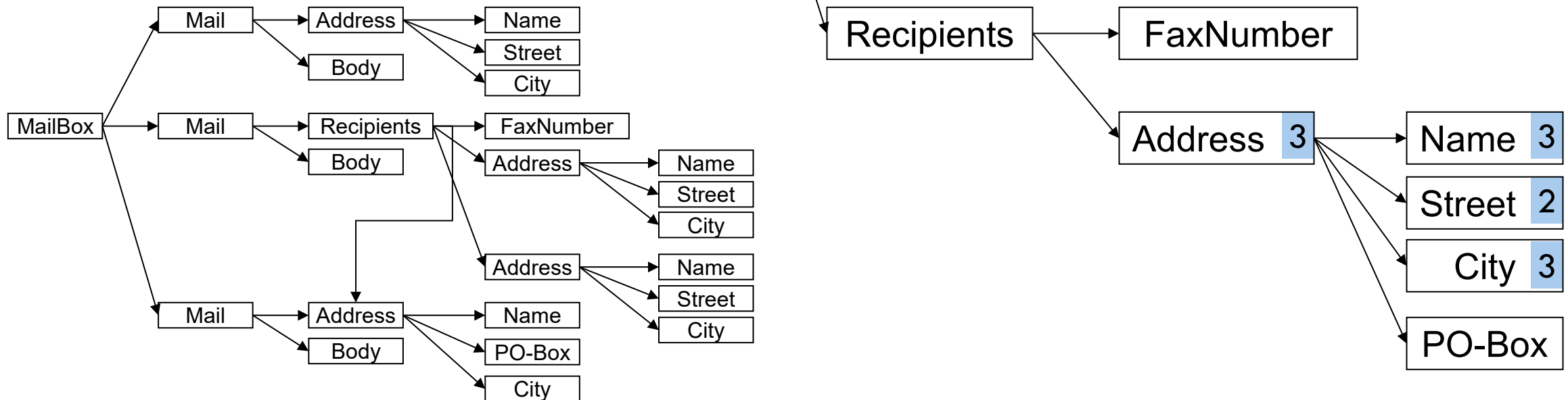
Memory Graph
