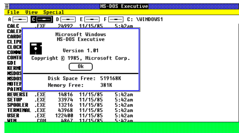
Windows 1.01
