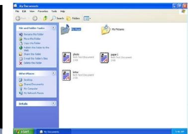
Windows XP
