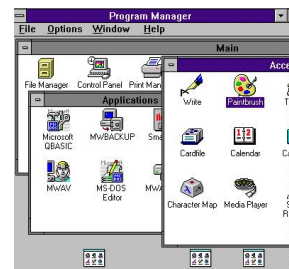
Windows 3.0
