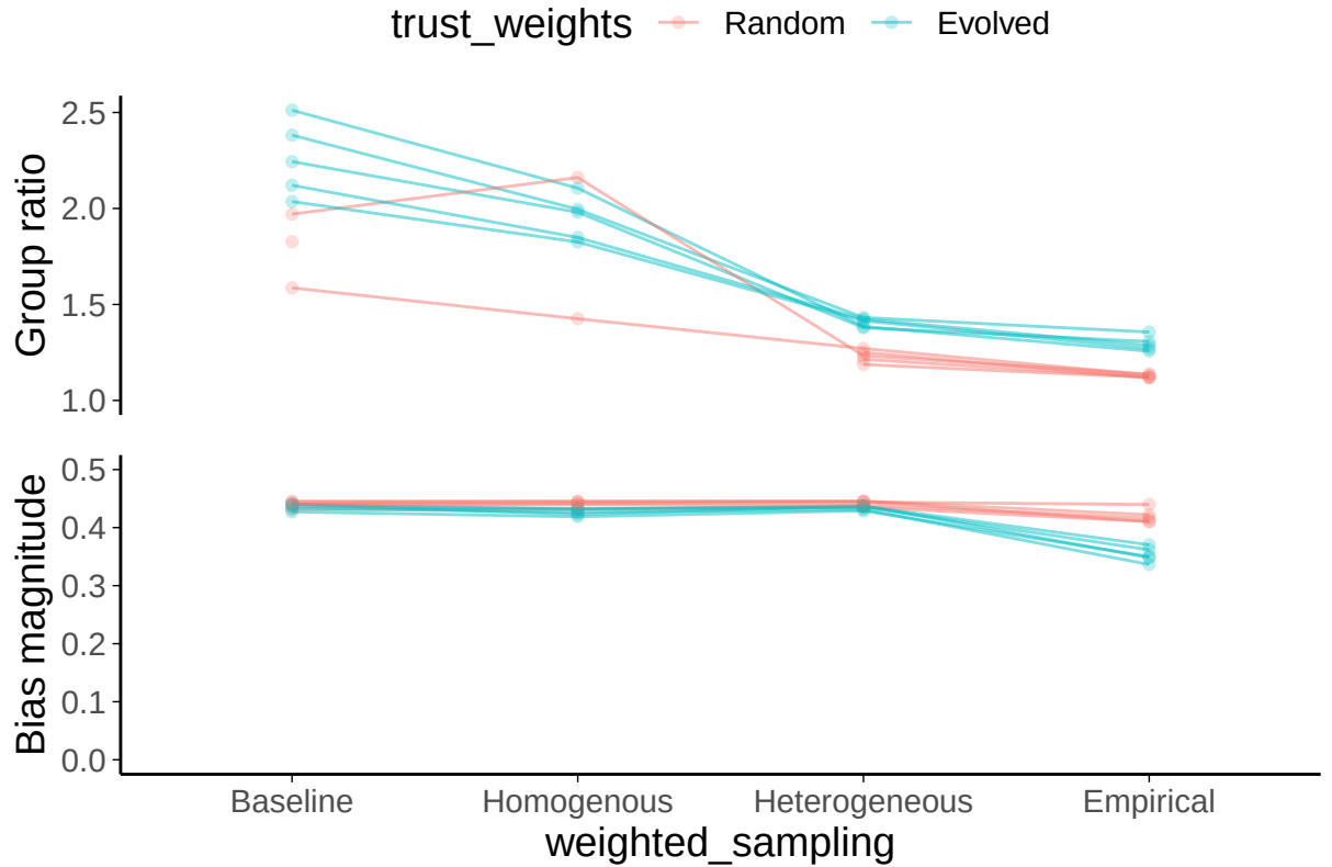
Figure 6.7: Model final decision group ratio and mean final bias magnitude.
