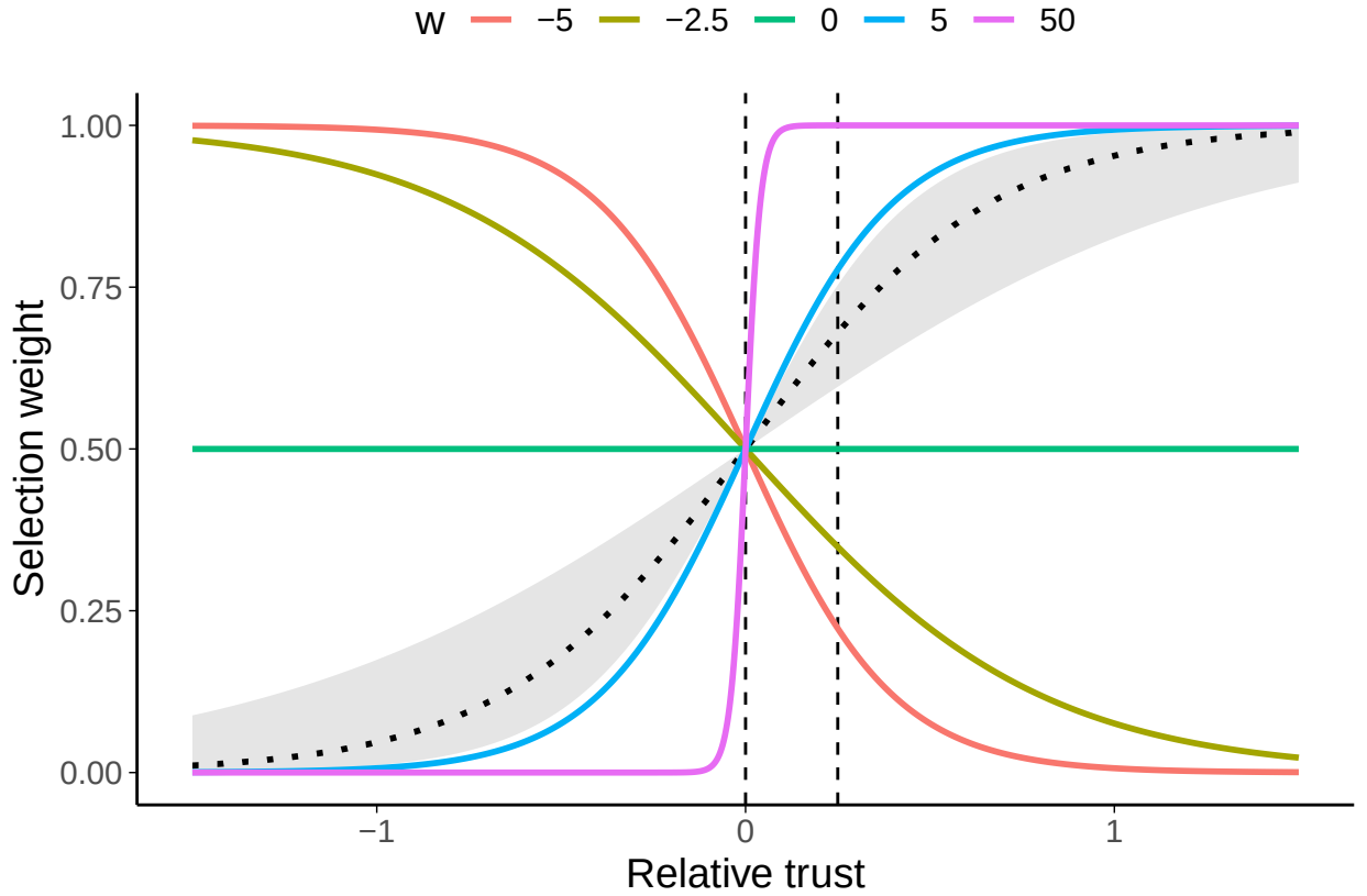
Figure 6.1: Weighted selection parameter.
