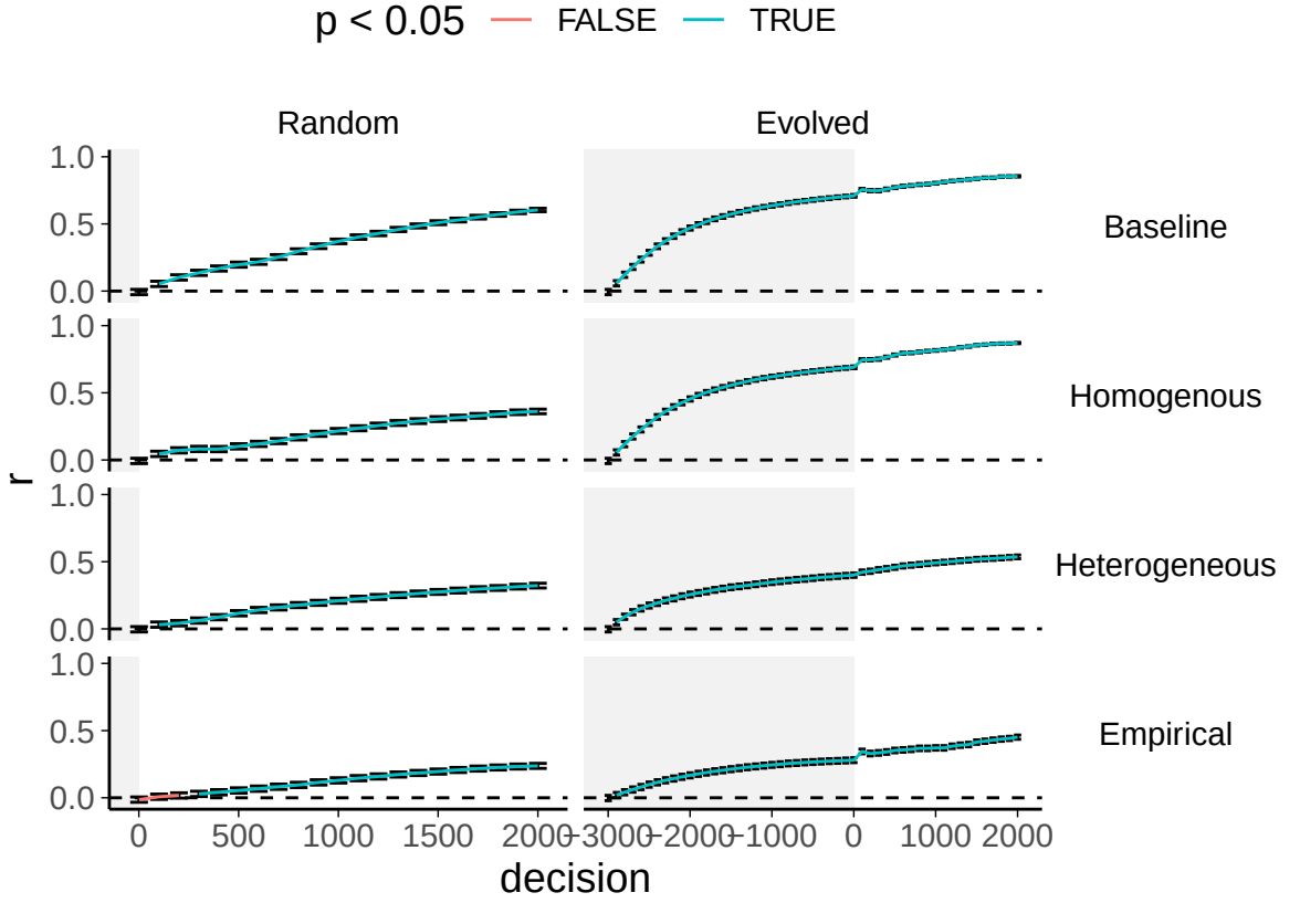
Figure 6.5: Shared bias-weight correlation evolution for each model.
