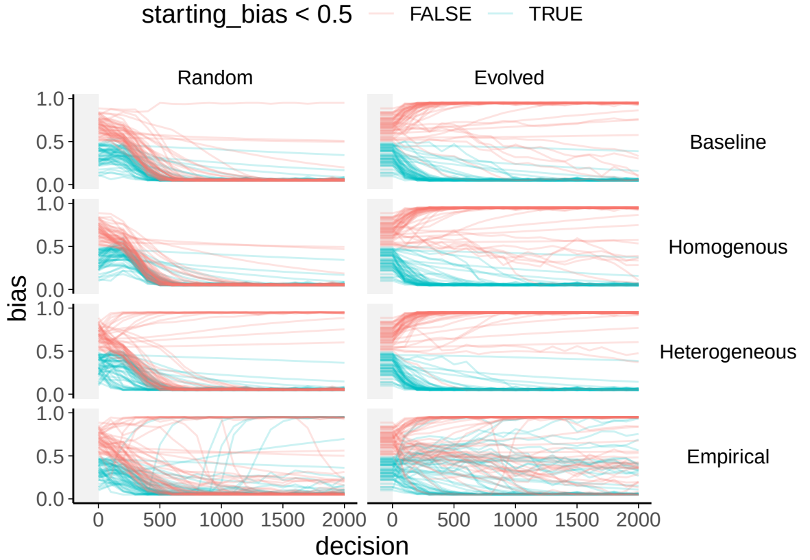
Figure 6.4: Bias evolution within each model.
