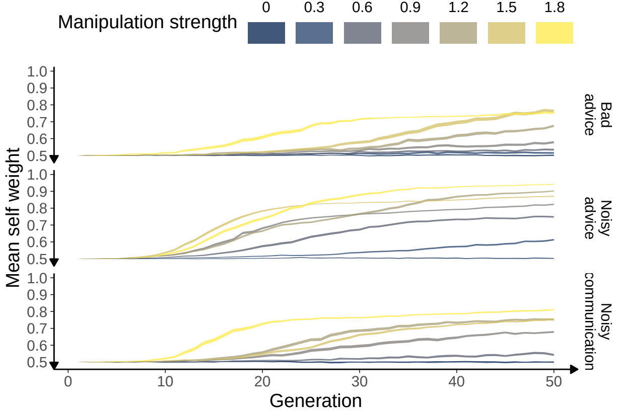
Figure 8.1: Egocentric discounting simulation results.
