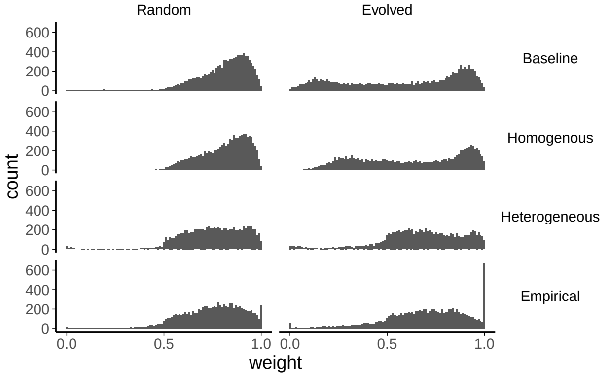
Figure 6.6: Distribution of final weights for each model.
