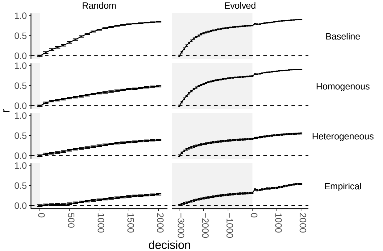
Figure 4.6: Shared bias-weight correlation evolution for each model.
