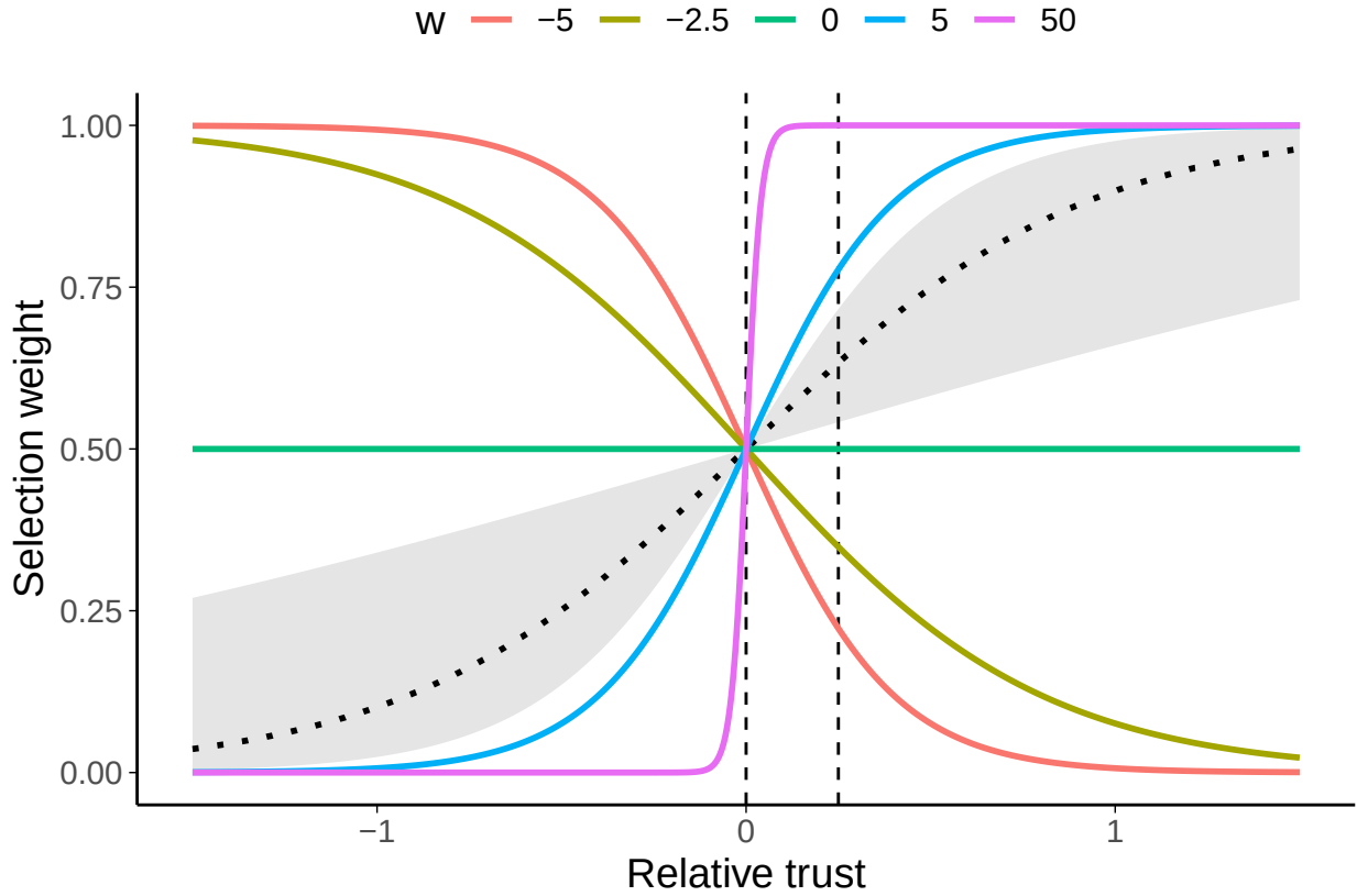
Figure 5.1: Weighted selection parameter.
