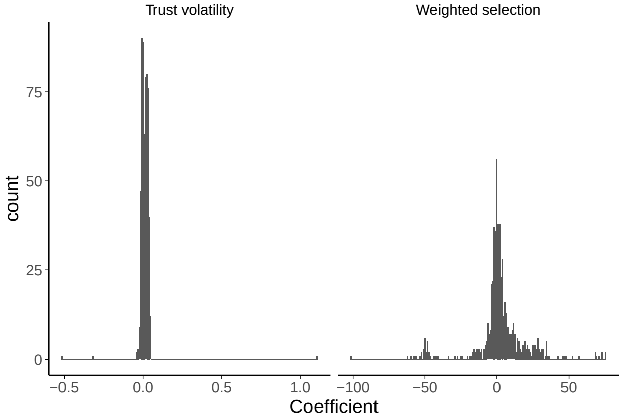
Figure 5.3: Histograms of recovered parameters.
