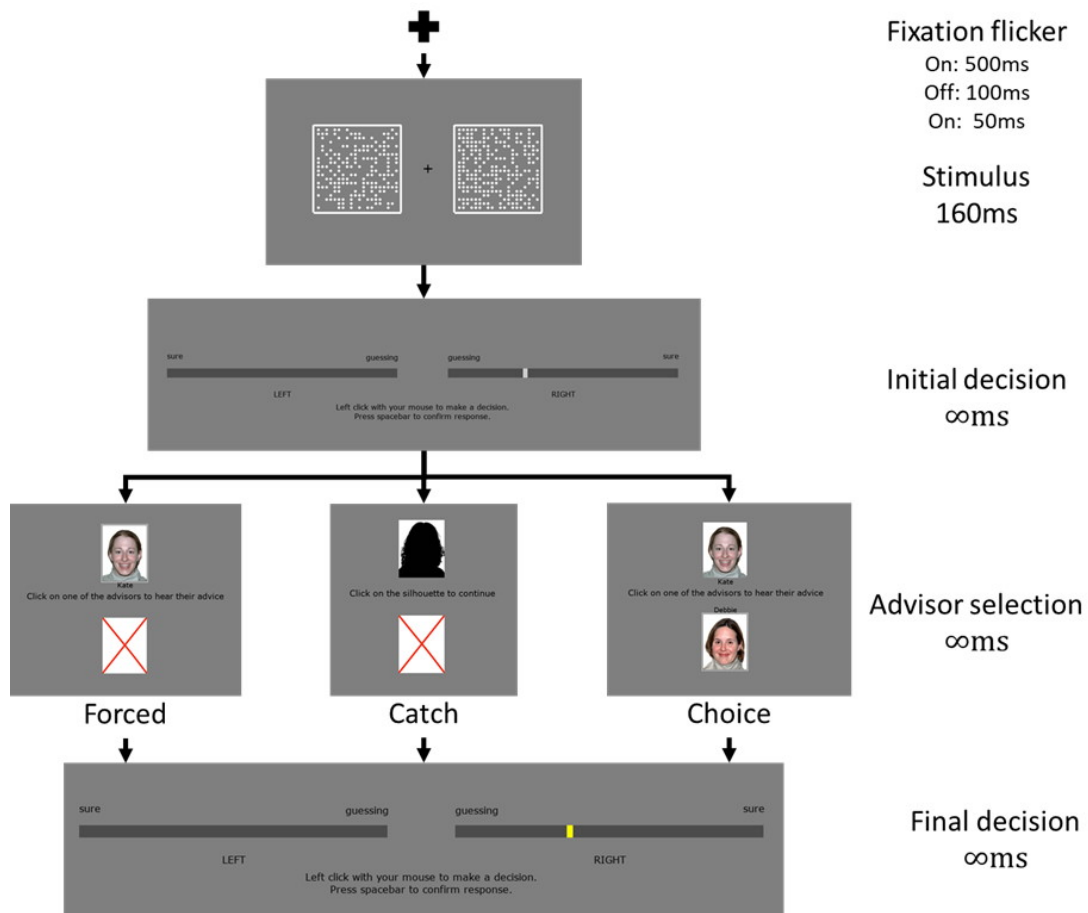
Figure 5.24: Experiment 1 procedure.
