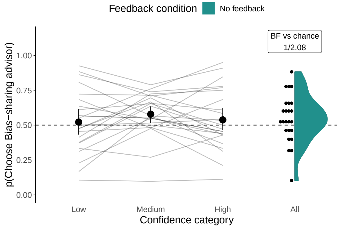
Figure 5.26: Advisor selection.
