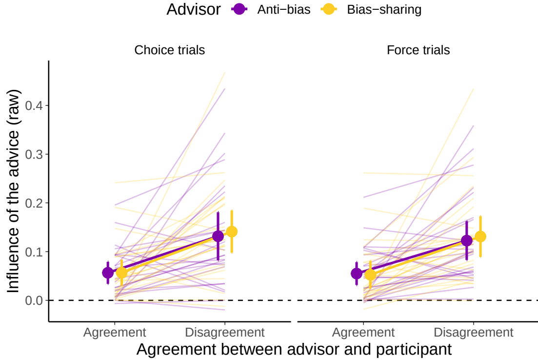
Figure 5.27: Advisor influence.
