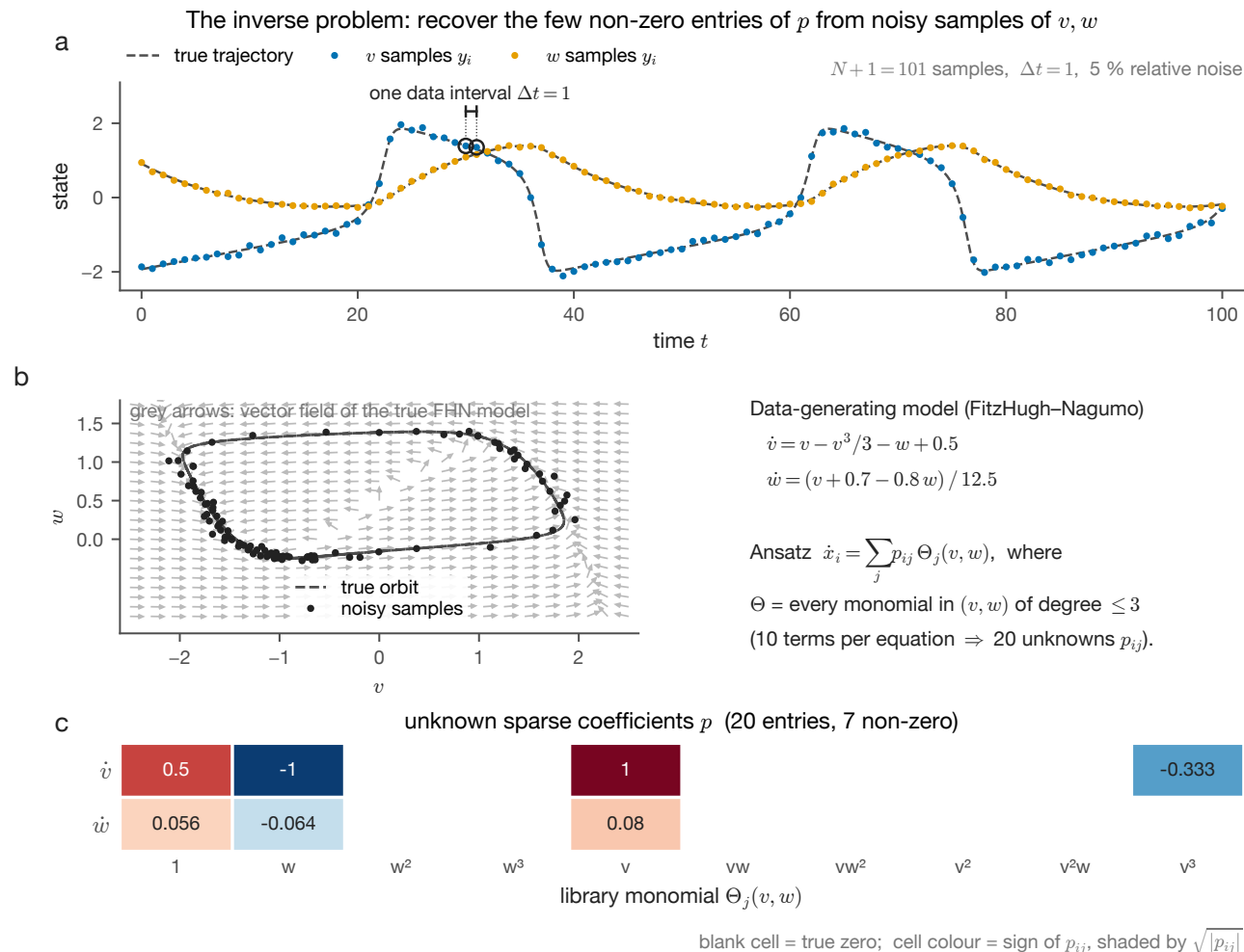
Figure 1: The inverse problem. (a) The FHN states v(t) (blue) and w(t) (orange) with the N = 101 noisy samples (dots) at spacing \Delta t = 1 ; the thin dashed line is the exact trajectory. (b) Phase plane with the vector field (light arrows), the true orbit and the noisy samples. (c) The unknown 2 \times 10 coefficient matrix over the monomial library \{1, w, w^2, w^3, v, vw, vw^2, v^2, v^2w, v^3\} : only 7 of 20 entries are non-zero (values shown). The task is to recover the non-zero pattern and the values from the dots in (a). Data: fhn_data.csv , fhn_fine.csv , fhn_vector_field.csv , fhn_library.csv .
