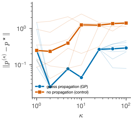
a Lotka–Volterra (12 coefficients, 5 % noise)
