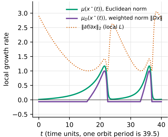
(c) Local rates along the FHN orbit
