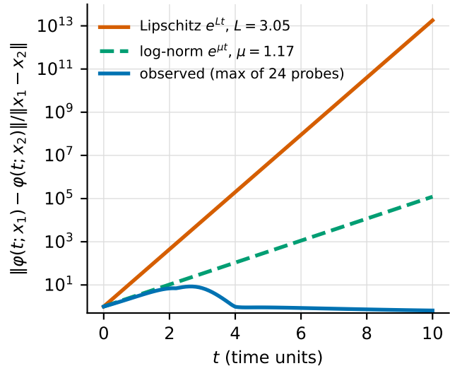
(a) Lemma 1: initial-state sensitivity
