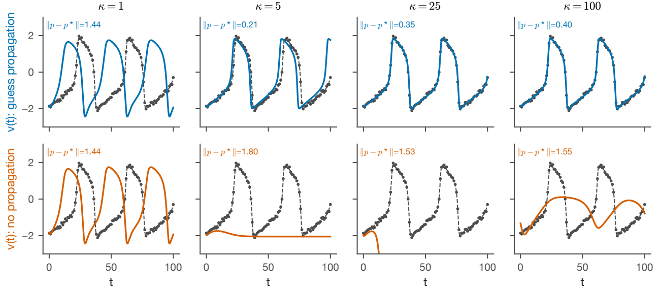
Figure 18: Filmstrip of the sweep (seed 2). Single-shooting simulation of v(t) from the minimiser returned at \kappa = 1, 5, 25, 100 (columns) for GP (top, blue) and the control (bottom, vermilion); grey dashed = truth, dots = data; the parameter error is printed in each panel. The GP fit tracks the data at every stage; the control loses the trajectory as soon as the windows are long. Frames of figures/anim_sweep.gif . Data: sweep_fits.csv , sweeps.csv .
