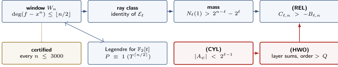
Figure 1: The reduction chain. Blue arrows are proved implications; the two red boxes are the open sufficient statements, either of which closes the chain. The gold box is the finite verification, which is insurance and not evidence for the open step. The double arrow records that the window question is Legendre’s conjecture for \mathbb{F}_2[t] , so no argument blind to the centre of the interval can separate them (Section 4, Barrier IV).
