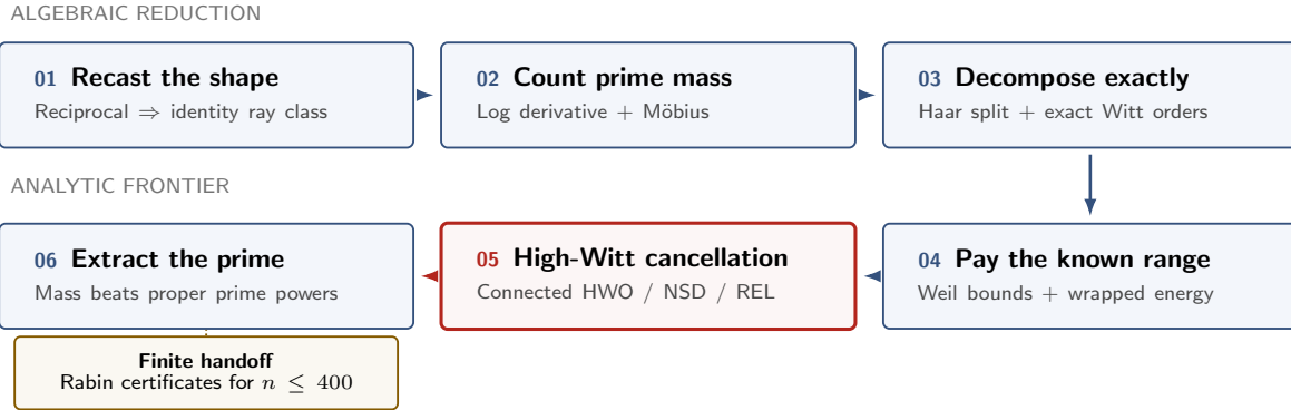
Figure 1: The current proof architecture. Stages 1–4 and 6 are proved; Stage 5 is the sole load-bearing open estimate. Gold denotes finite verification.
