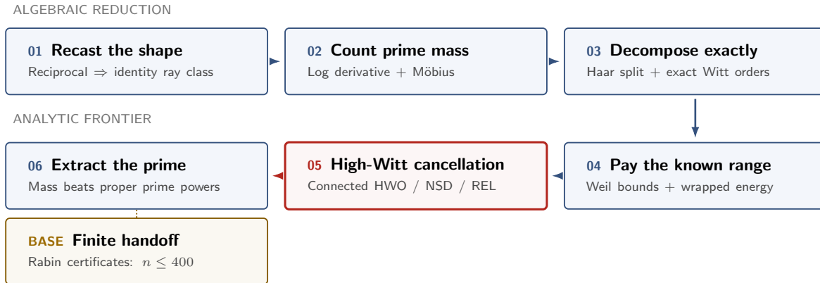
Figure 1: The current proof architecture. Stages 1–4 and 6 are proved; Stage 5 is the sole load-bearing open estimate. Gold denotes finite verification.
