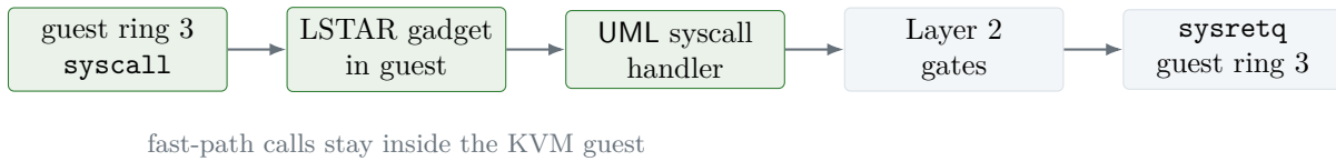
Figure 5: kvm-v2 fast syscall shape after gadget revival. Trivial syscalls avoid a host vmexit on the hot path.
