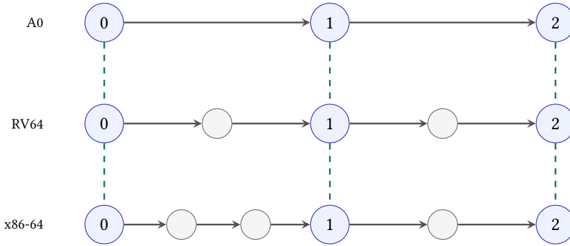
Figure 12.3: Forward simulation relates synchronization points, not every row. One Ao segment can match several RV64 or x86-64 instructions.
