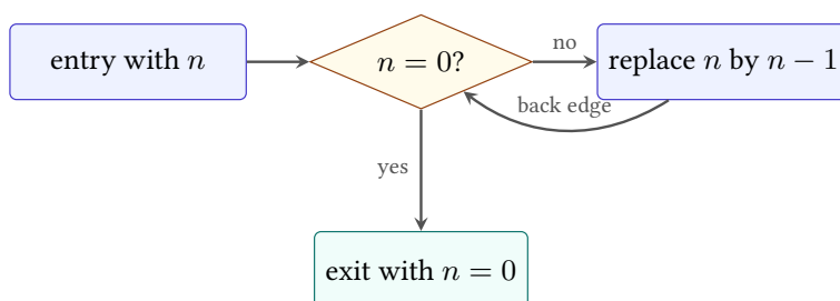
Figure 9.3: The common mathematical control shape beneath the three listings. The machine-specific predicates and target conventions implement these edges.
