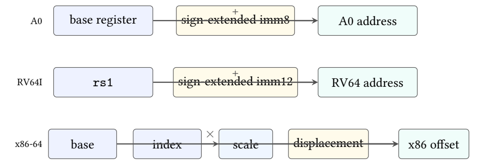
Figure 7.1: Selected effective-address shapes. Ao and RV64I use one base and a sign-extended immediate. A selected x86-64 form can combine base, scaled index, and displacement. Every result still needs a validity check before access.
