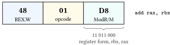
Figure 6.4: One three-byte x86-64 encoding of add rax, rbx . The byte boundaries are regular here; the instruction family as a whole is not fixed at three bytes.
