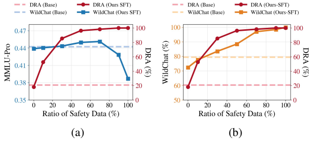
Figure 3. Impact of safety data scaling. (a) Increasing safety data yields initial gains but ultimately degrades general performance due to over-alignment. (b) Higher safety ratios consistently strengthen reflective defenses against overtly harmful queries.
