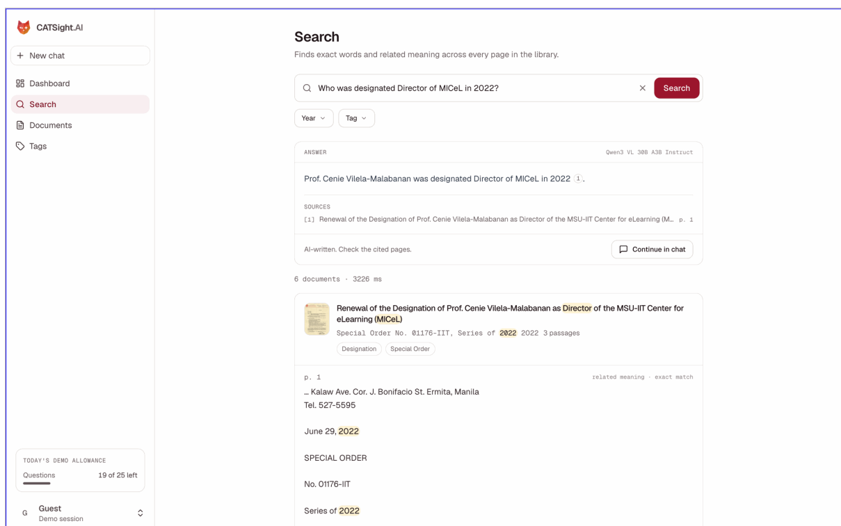
Figure 6.4. A Question in the Search Page, with a Short Cited Answer
