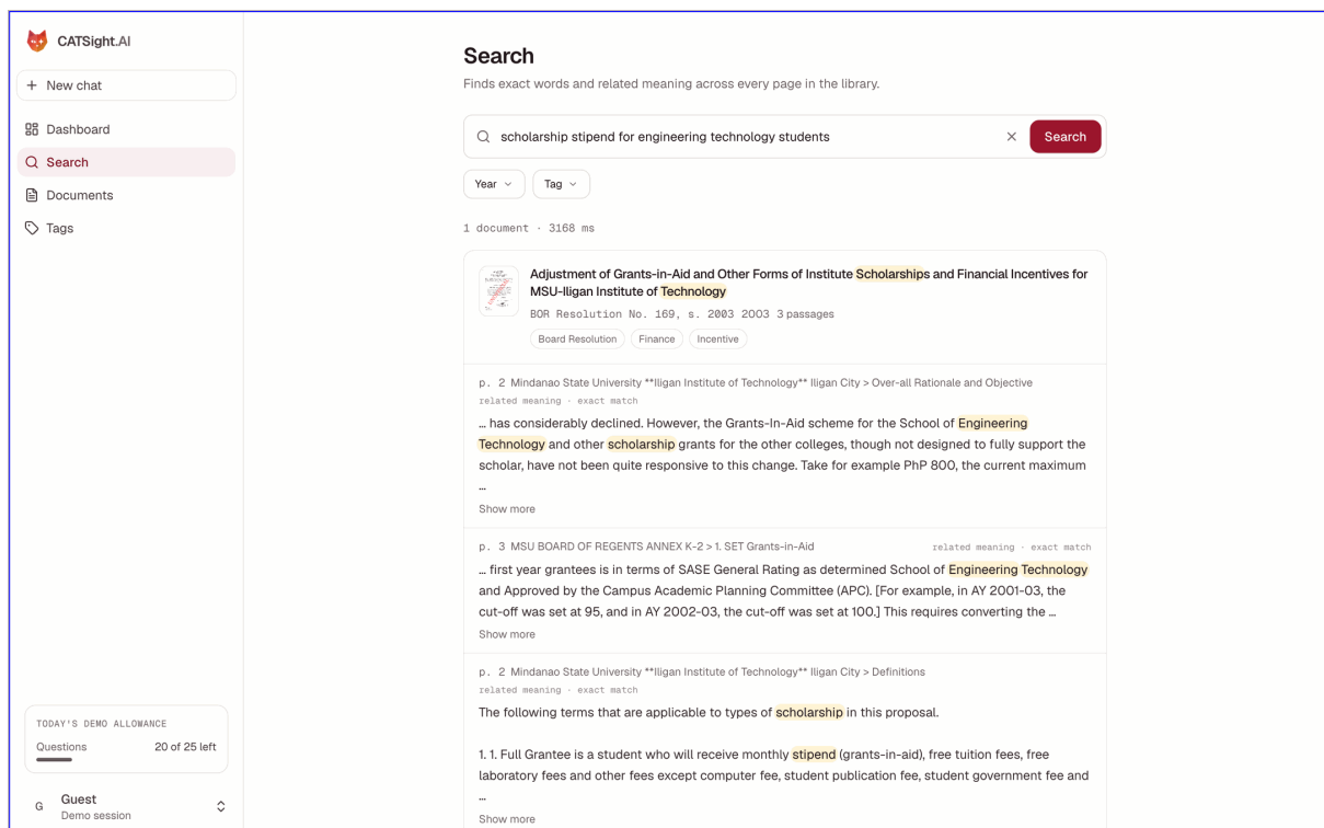
Figure 6.3. Search by Meaning: a Paraphrased Query Finds the Grants-in-Aid Resolution
