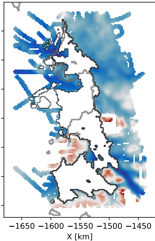
(b) BedMachine terrain effect
