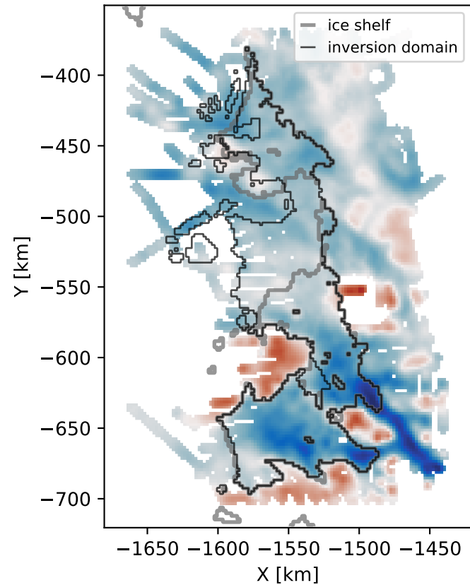
(a) Observed gravity disturbance
