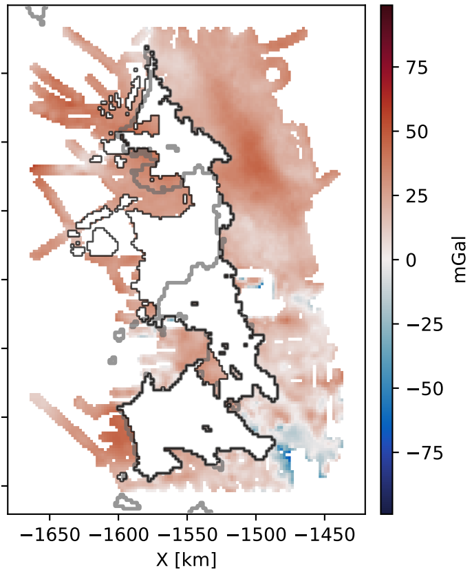
(c) BedMachine Bouguer disturbance
