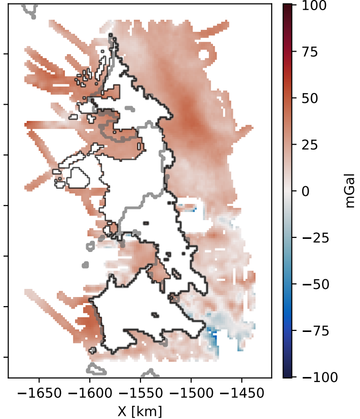
(c) BedMachine Bouguer disturbance
