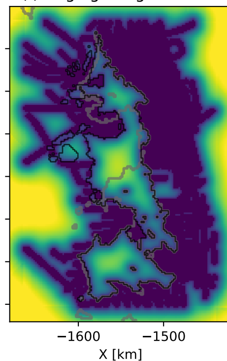
(f) Kriging Bouguer stdev
