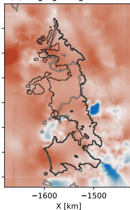
(e) Kriging Bouguer mean
