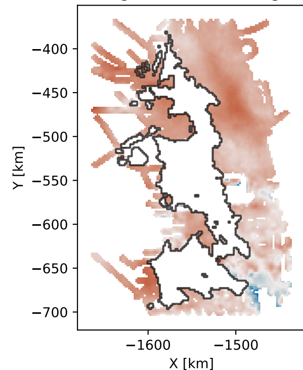
(c) SGS Bouguer realization 1
