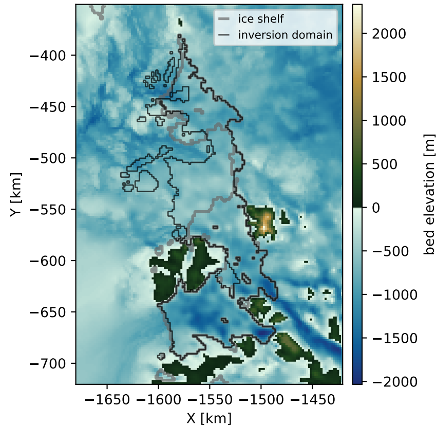
(a) BedMachine bed
