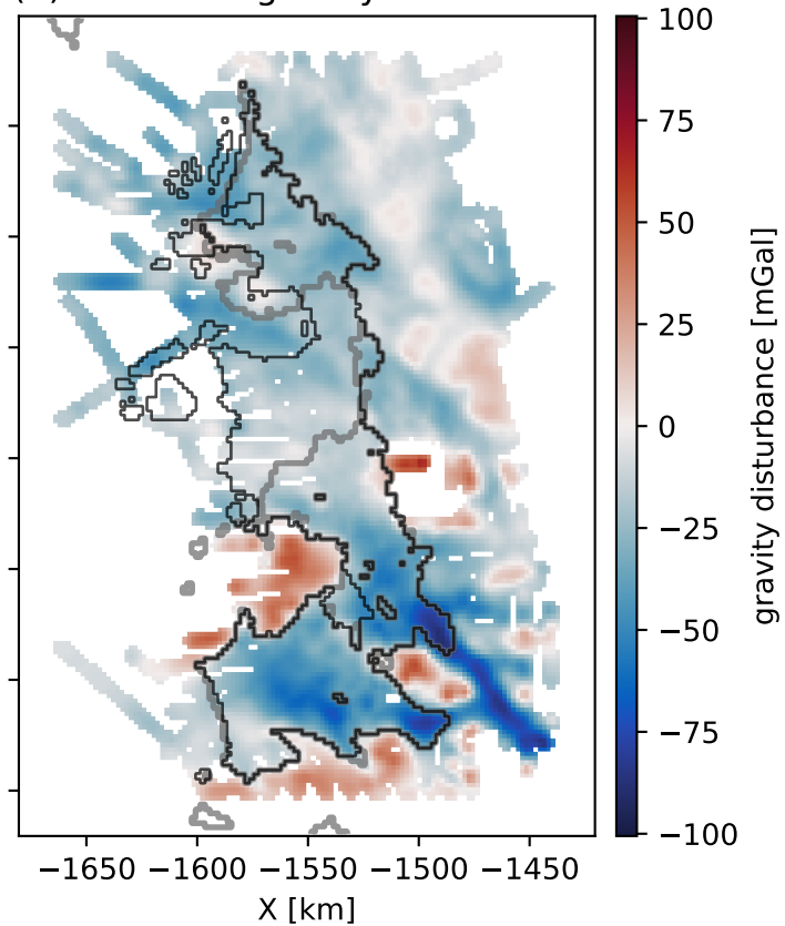
(b) Observed gravity disturbance
