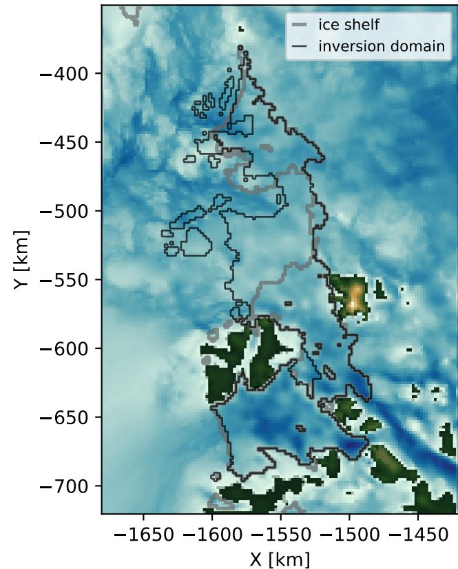
(a) BedMachine bed
