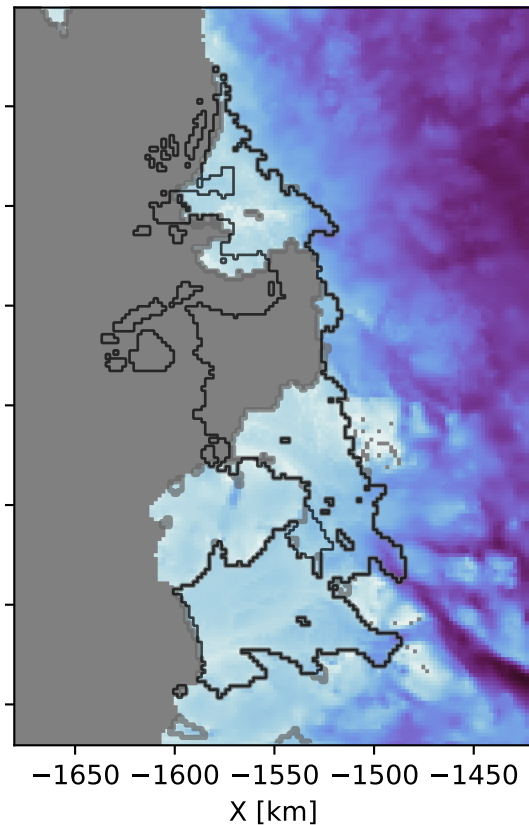
(b) BedMachine thickness
