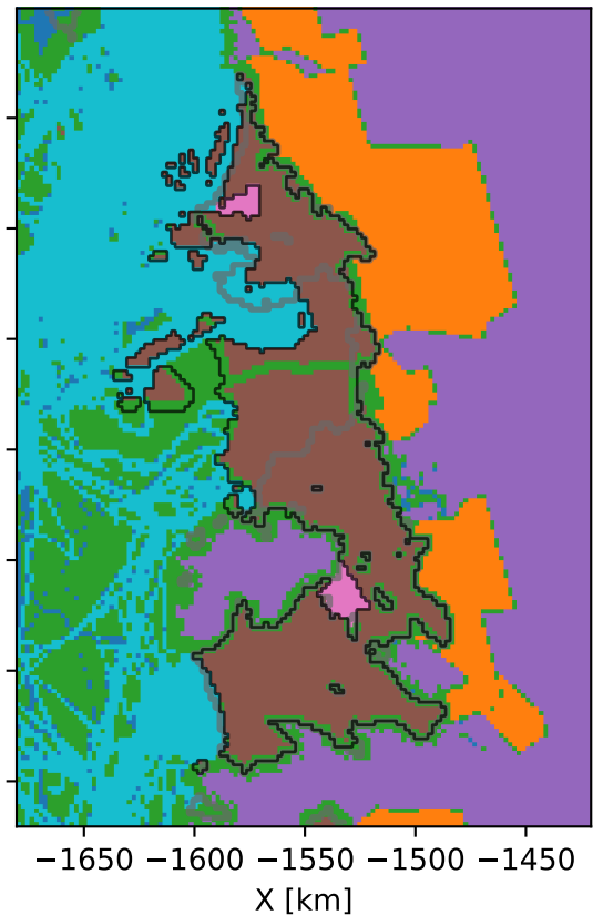
(c) BedMachine source
