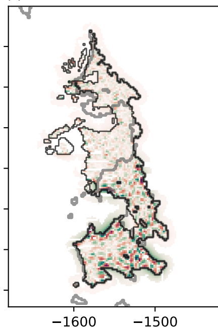
(f) Inversion residual mean
