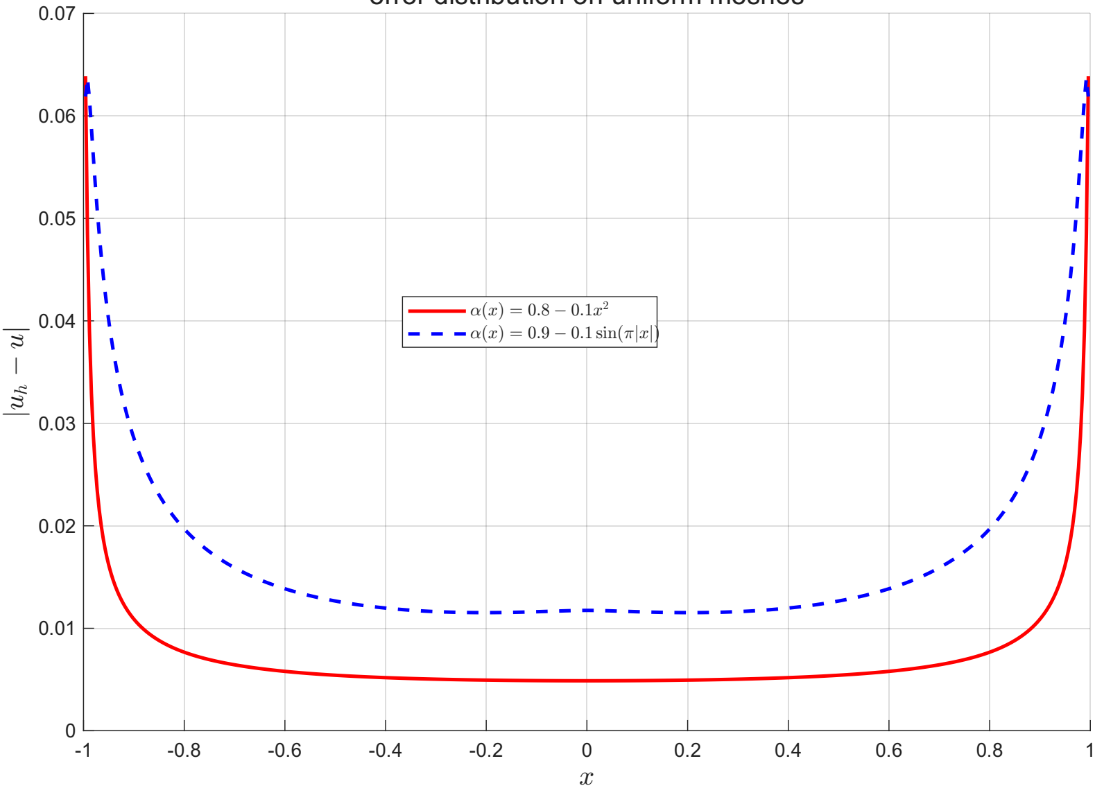
error distribution on uniform meshes
