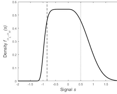
Figure 2: Asymmetric distribution of taste shocks f_{\alpha_L, \alpha_H} , for \alpha_L = 10, \alpha_H = 2.5 .
