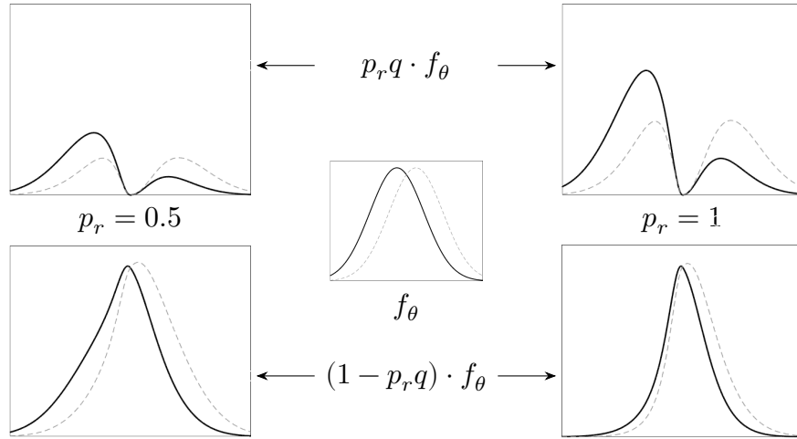
Figure 4: Distributions of reviews for f_\theta(s) normal, with \frac{\mu}{\sigma} = 0.25 , and q(s) = 1 - \frac{1}{1+2(x^2+4\mathbb{1}_{\{x \leq 0\}}x^2)} and for p_r = 0.5 (left), 1 (right). The top panels show the distribution of submitted reviews, and the bottom panels show the distribution of null reviews.
