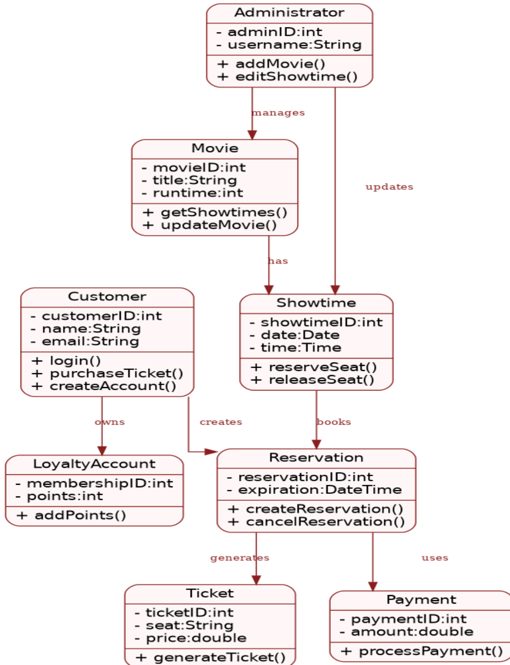
Figure 2. UML Class Diagram
