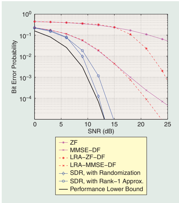
[FIG3] Bit error probability performance of various MIMO detectors in a QPSK 40 \times 40 MIMO system. Zero forcing (ZF), minimum mean square error (MMSE), decision feedback (DF), lattice reduction aided (LRA). “Performance lower bound” is the bit error probability when no MIMO interference exists.
