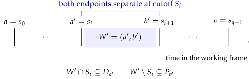
Figure 1: One side of a node, viewed in its working frame. Each nonempty gap uses the cutoff belonging to its strict walk step. The endpoints separate that same cutoff, although adjacent gaps may use different cutoffs. The horizontal arrow denotes schedule time, not a precedence relation.
