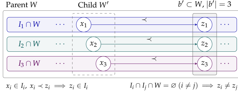
Figure 2: Why at most three injections survive a same-direction update. For each surviving injection, choose a high job x_i in the child and a successor z_i in its ending triple b' . Upward closure puts z_i in the same injection; disjointness on the parent W makes the chosen z_i distinct. The three-injection case is drawn; arrows denote precedence. Only witness pairs are shown: the injections may contain other jobs and may overlap outside W .
