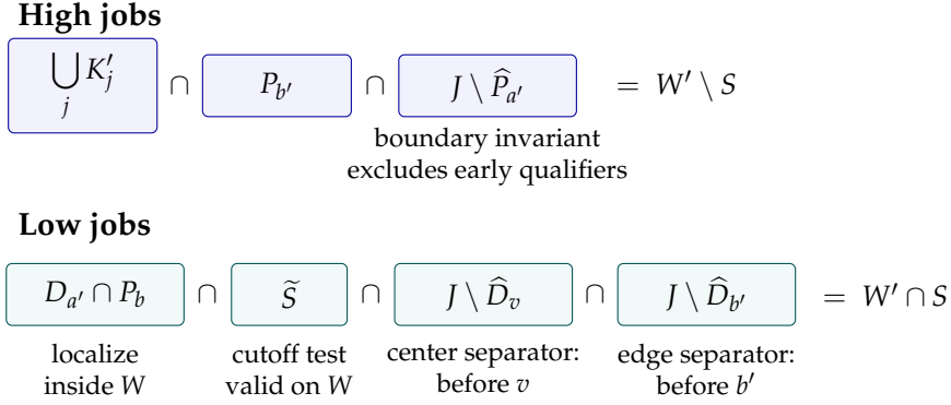
Figure 4: The two global tests for a child. For the low part, positive cones locate a candidate inside the parent before its cutoff predicate is used; the two weak successor exclusions then restrict that candidate to the gap. For the high part, the global past-boundary invariant excludes qualifiers at or before a' . The intersection factors are arranged in the order used by the proof.
