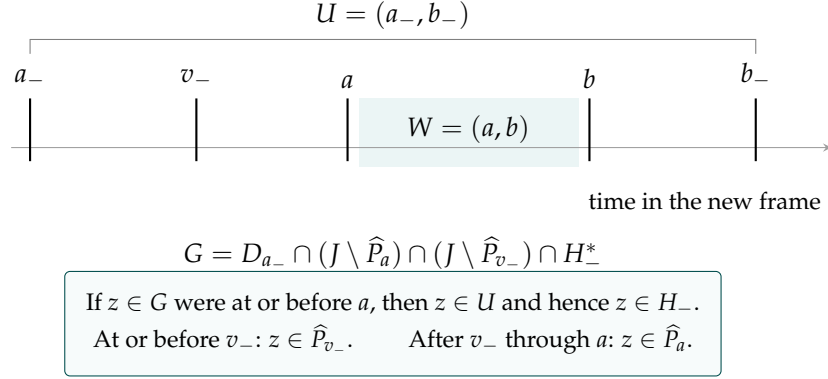
Figure 3: The ancestor configuration at a direction change, in the new working frame. A candidate early member of G is first located inside U by D_{a_-} ; only there is the earlier cutoff extension used. The two weak predecessor exclusions then cover the portions at or before v_- and between v_- and a . The equality a = v_- is allowed; the intervening segment then collapses. The horizontal arrow denotes time.
