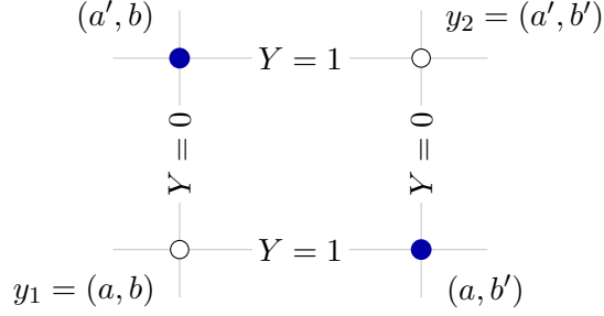
Figure 2: Two candidate center states differing in both coordinates admit exactly two point states in their common strict cross. The filled points are those opposite corners. Within this four-state configuration, the bit of a consistent edge and the state at either endpoint determine the state at the other endpoint. Rows have fixed first label and columns have fixed second label. The diagram displays coordinate equalities of states, not geometric positions of the original plane points.
