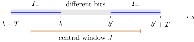
Figure 1: The intervals I_- = [b - T, b] and I_+ = [b', b' + T] , with b \leq b' and T \geq 0 , flank the bit-difference interval. The central window J in Theorem 5.4 creates excess only if its total overlap with the two flanks exceeds T ; then both thresholds lie strictly inside J .
