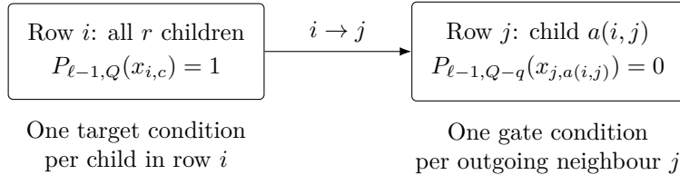
Figure 1: One recursive clause. The edge label selects a single child in each outgoing neighbour's row. Raising q strengthens the gates; all targets use the strongest child predicate Q .
