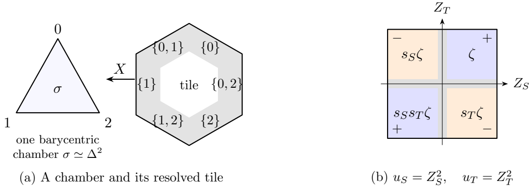
Figure 1: The reflected resolution in dimension two, following Gaifullin's permutohedral construction [7]. In (a), one barycentric chamber \sigma \simeq \Delta^2 is paired with its resolved tile. The six facets are indexed by the nonempty proper subsets of \{0, 1, 2\} ; adjacent labels are nested. The map X sends the tile interior diffeomorphically to the chamber interior. In (b), at a corner with labels S \subset T , a full state \zeta = (\sigma, p, t) and its three reflected states occupy the four quadrants of signed coordinates. The commutation s_S s_T = s_T s_S and the independent bit toggles give four distinct quadrants of one smooth chart. The displayed signs compare each chamber sign with that of \zeta : blue agrees and orange is opposite. The gray collar and strips represent the same seam schematically; their widths are illustrative, and X is not affine.
