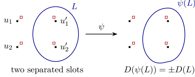
Figure 5: Nearby nails (squares) detect the separations of endpoint pairs (dots). The homotopy bijection preserves oriented winding differences. A single sign change of a loop's whole separation vector cancels when that loop occurs an even number of times.
