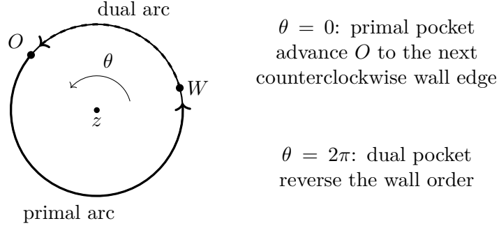
Figure 4: Normalized chart of a two-change component. The angle \theta = O - W is measured counterclockwise along the dual arc. The arrows on the circle indicate boundary order, not strand orientation. The forcepoint reset uses the next old-wall edge on the retained pocket. A full turn changes the endpoint of the reflected angular interval. The drawing is schematic; microscopic tip and force sides are suppressed.
