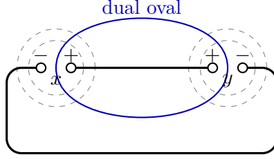
Figure 6: The bulk gluing used in the lower bound. Black connections join the positive terminals and the negative terminals separately; the dual oval keeps these two actual primal clusters distinct. Each terminal is protected by a small primal circuit. Only connectivity is depicted; the four-arm annuli are schematic.
