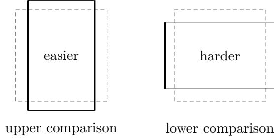
Figure 3: The Jordan-quad comparison in Schoenflies coordinates. The dashed square is the limiting target; thick sides are separately wired electrodes. The easier quad extends beyond the free sides and ends inside the target's electrode sides. The harder quad has the opposite inclusions. Physical test polygons retain strict margins after pullback and lattice approximation.
