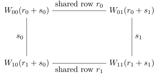
Figure 1: A square after fixing the slice background. The four rows r_0, r_1, s_0, s_1 are independent, but their four sums satisfy one parity relation. Fourier expansion therefore leaves one common frequency. Different squares of a collision-free cube use disjoint rows.
