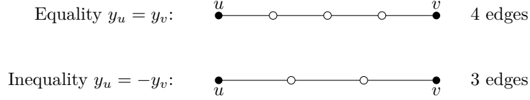
Figure 2: Each unit demand becomes a path with fresh internal vertices. For fixed endpoint signs, its minimum uncut cost is zero if the demand holds and one otherwise. Identifying the endpoints gives a four-cycle or a triangle and handles self-demands with the same exact cost.
