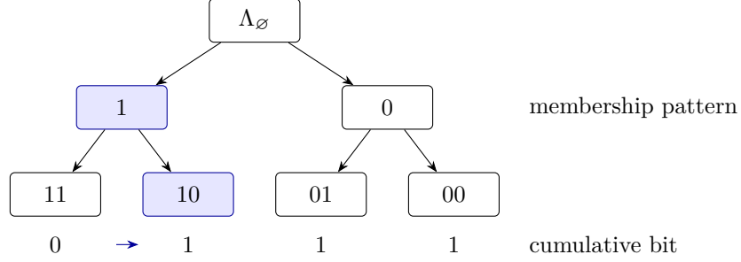
Figure 1: Schematic transition refinement for two prefix slots. Membership 1 precedes 0 lexicographically. In the illustrated case the cumulative bit changes at cell 10, so the transition is in the first cell at depth one and its second child at depth two. The selected membership bits are therefore f_{u_1, \mathcal{D}_0}(P_1) = 1 and f_{u_2, \mathcal{D}_1}(P_2) = 0 , with each function using its preceding prefix. Empty cells are retained in the ordering but cannot contain a transition.
