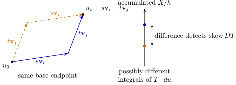
Figure 2: Two orders of the same two base displacements. The difference between their line integrals has mixed term st(DT(u_0)[\mathbf{v}_i] \cdot \mathbf{v}_j - DT(u_0)[\mathbf{v}_j] \cdot \mathbf{v}_i) . This is a schematic illustration of the obstruction; the proof uses 2m successive legs, with the first and last m directions forming bases.
