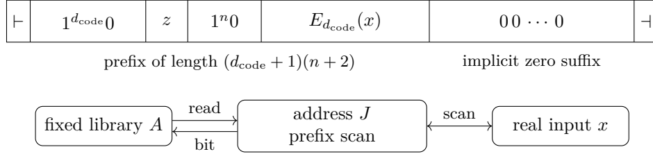
Figure 2: The fixed library reads the padded input through a callback. The callback regenerates prefix symbols from the real input and returns zero for an address in the padding interval.
