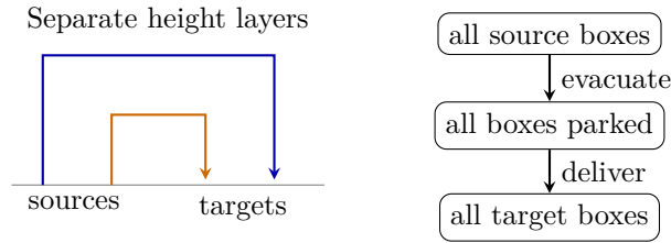
Figure 1: The two separation mechanisms in Lemma 3.3. Left: horizontal projections separate the lift and descent, and distinct heights separate the transfer; the second horizontal coordinate is suppressed. Right: a temporal schedule, not a spatial drawing. Every source is removed before any target is occupied, so overlap between the two families is harmless.
