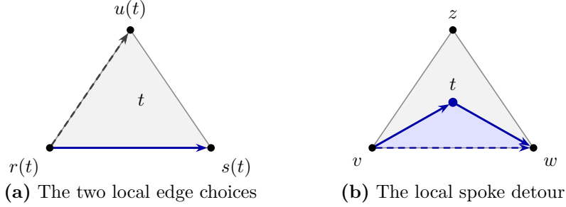
Figure 1: Two local constructions in a bounded black triangle. (a) A paired state gives the edge r(t) \rightarrow s(t) of D (solid) and the edge r(t) \rightarrow u(t) of Q_s (dashed). (b) The directed edge v \rightarrow w (dashed) is slid to the two-spoke route v \rightarrow t \rightarrow w (solid), with t denoting the face center. The shaded subdisk lies between the two routes and excludes the third corner z .
