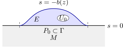
Figure 1: A local schematic cross-section of the common exterior cap. The boundary moves only over a compact subset of the measured patch. The oval is a nonempty open source set U_0 with closure inside E . The proof uses the smooth graph, including its flat bump edges.
