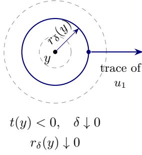
Figure 3: A normal-coordinate section of \gamma -geodesic spheres in the first variable, where \gamma is the conformal reference metric. The center y satisfies t(y) < 0 . The spatial dilation \lambda is fixed while \delta decreases. The Green functional transfers paired harmonic functions and reproduces affine harmonic coordinates exactly. The unit-sphere measure d\sigma_y has total mass one; the density \psi_\delta need not be positive.
