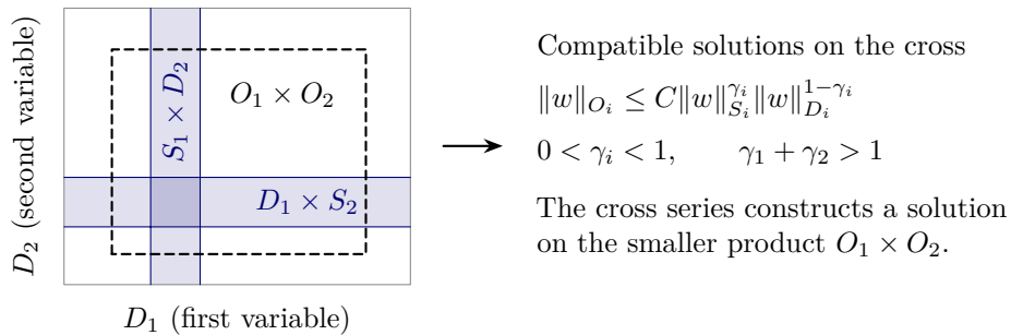
Figure 2: Compatible product solutions are given on the shaded cross. The L^2 interpolation estimates for single-variable solutions, with \gamma_1 + \gamma_2 > 1 , make the singular-function series converge on O_1 \times O_2 . The drawing is schematic: each factor is a multidimensional domain, and containment of S_i in O_i is not required.
