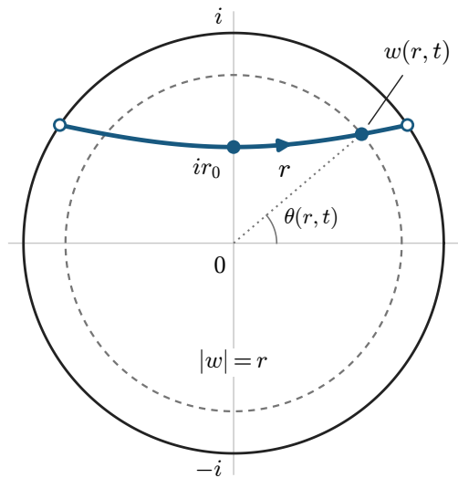
Unit disk \mathbb{D}
