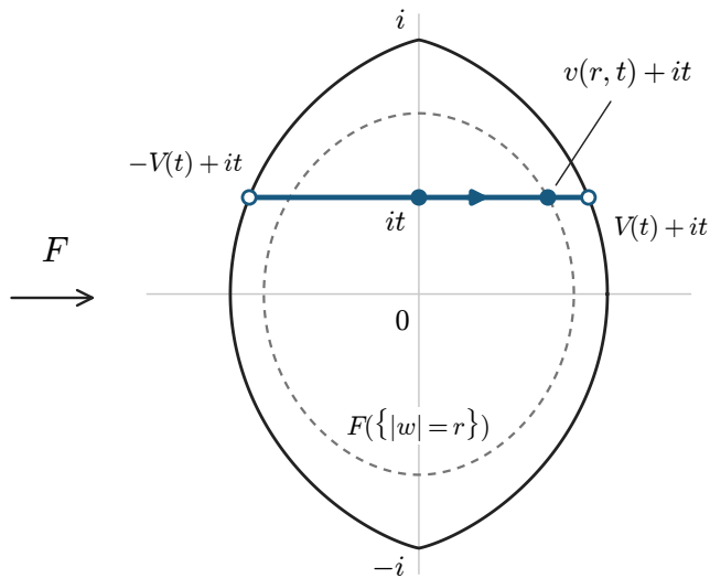
Image D = F(\mathbb{D})
