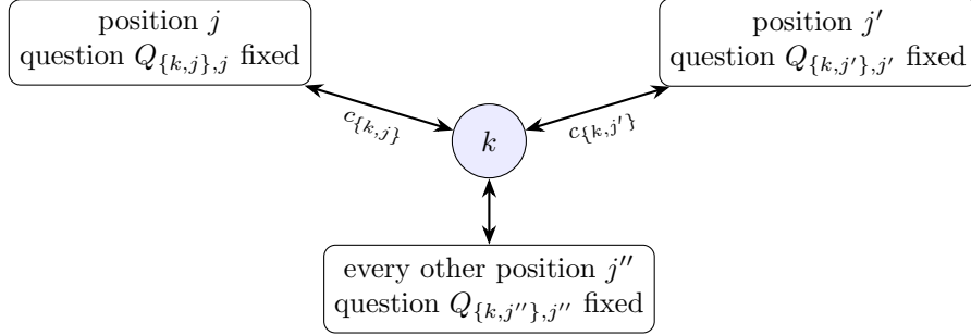
Figure 1: The star operation centered at k . Each incident seed is resampled within the fiber of its question at the opposite endpoint. All nonincident seeds and all weights stay fixed. Thus every query except the query at k stays fixed. The schematic depicts the conditional averaging operator D_k , not additional graph edges.
