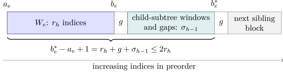
Figure 1: The block attached to an edge at height h \geq 2 , shown schematically. The window length is at least the length of the following gap and child-subtree span together. Thus the entire block has at most twice the window length, regardless of where it occurs in the tree. The next sibling block is outside this bound. At height 1, the child is a leaf and the block consists only of W_e .
