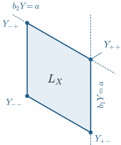
(a) Feasible witnesses in L_X
